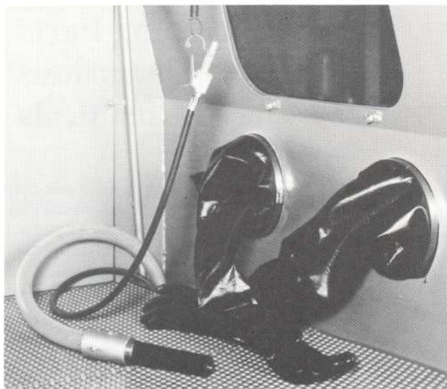
The cabinet interior features high-intensity lighting, a venturi blast nozzle with lightweight blast hose, a dust-off gun and abrasion-resistant operator gloves.
