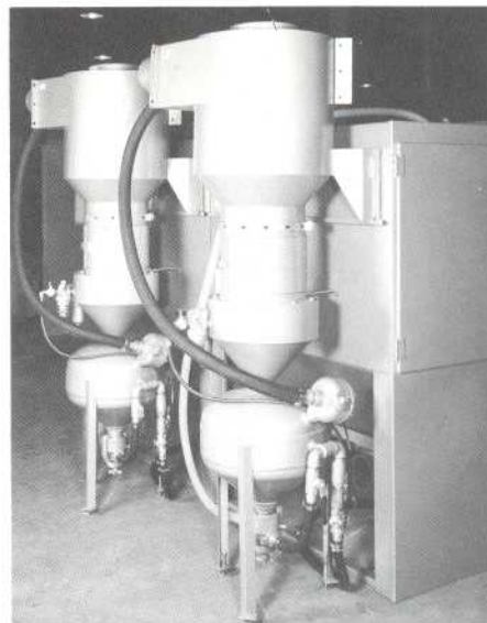
FaStrip cabinets are equipped with an automatic Sure-Flo media regulator, a MG-78 CR exhaust valve and a vibrating screen within the reclaimer to assure smooth, consistent flow of lightweight plastic abrasives.
